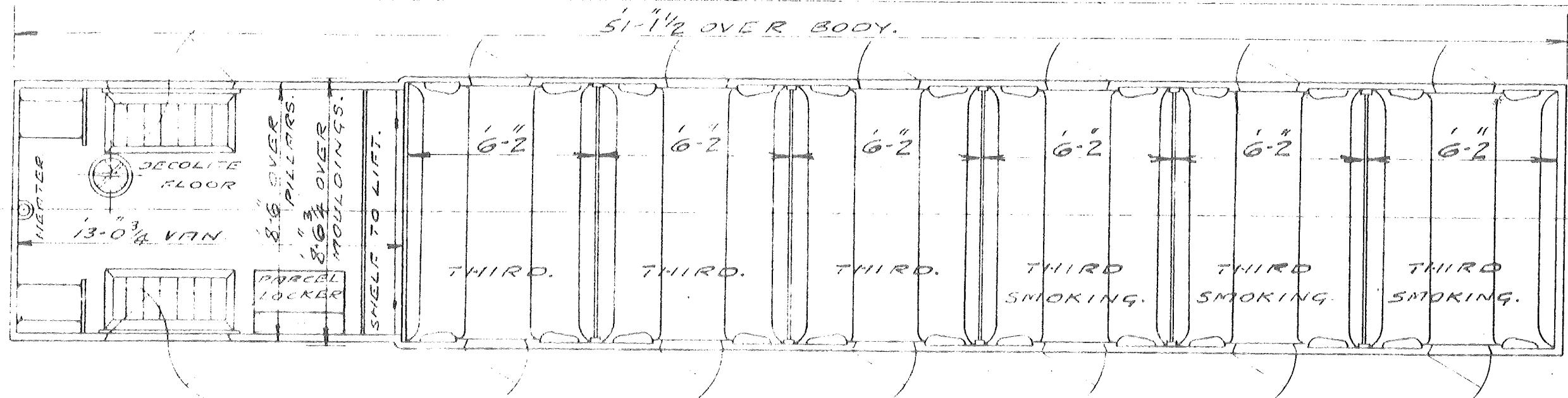
C.L.C. THIRD CLASS BRAKE.
